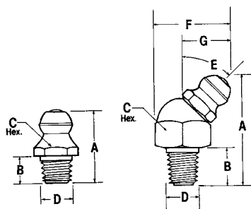
No. 205410 1/4" -28 Spec. Taper Drive Th'd.
