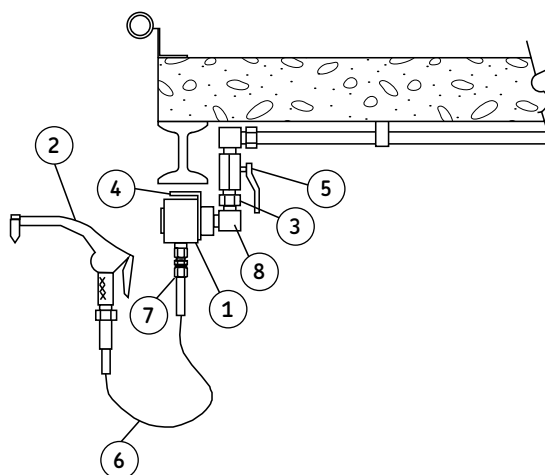
Chassis control valve
