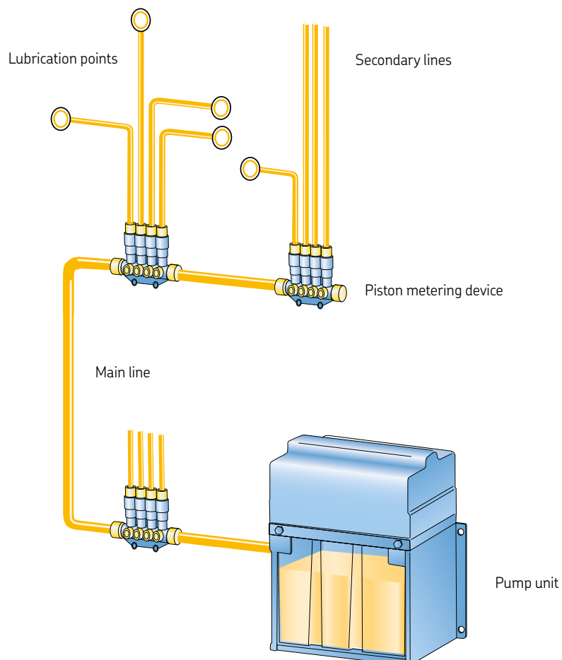
SKF MonoFlex lubrication systems for mobile on-road
