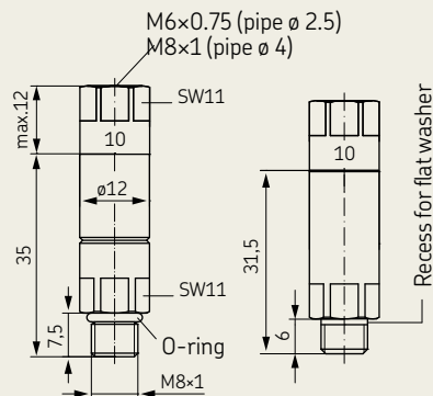
Dimensions: Product series 341 + solderless pipe connection (00)
