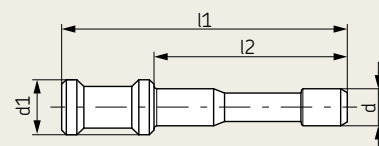
Locking pin
