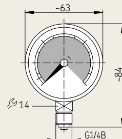
Pressure gauge
