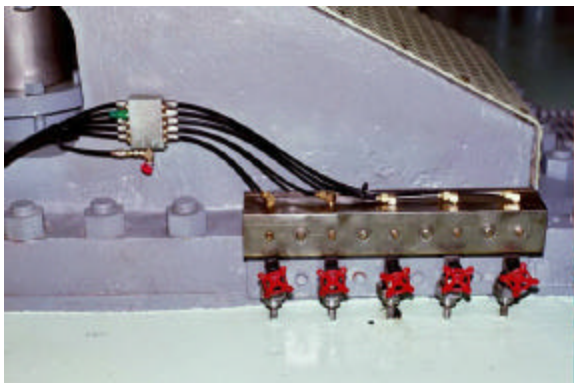
Close up of Divider Valve with lines going into five grease points on each side of the gate.
