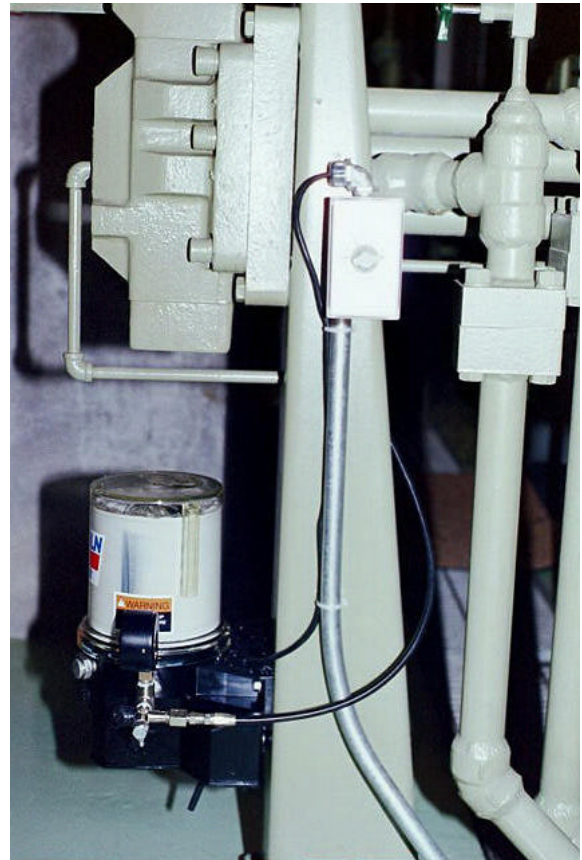
View of pump and controller mounted on support bracket next to a gate. As the gate is moved, the system is activated lubricating the slides of the gate. The system can be installed during gate operation.
