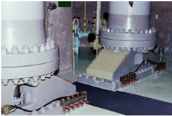
Two gates showing divider valves metering grease to each individual point.
